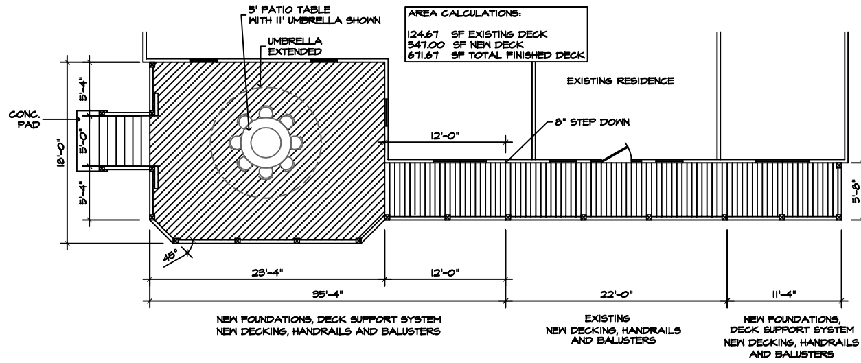
PROPOSED DECK PLAN
