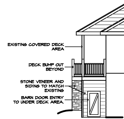
PROPOSED RIGHT ELEV
